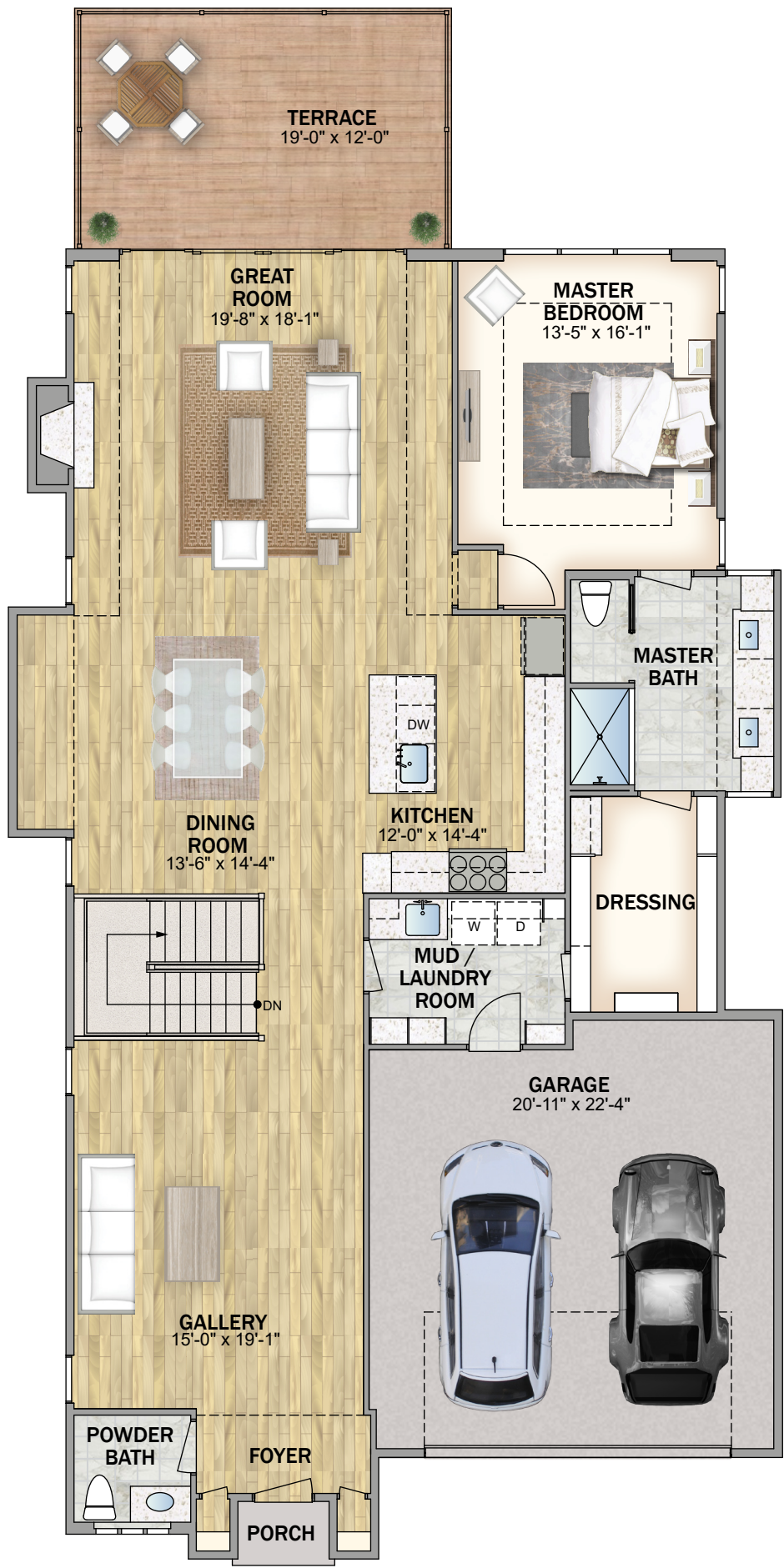
PLAN A - FIRST FLOOR
